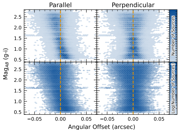
Figure 26. Visualization of Differential Chromatic Refraction (DCR) observed in the LSSTComCam commissioning campaign. The g-i color is computed for every source in the reference catalog that is matched to a direct source in the science image, and the binned density for the full survey is plotted against the angular offset between the reference and detected positions. The angular offset is projected along coordinates parallel and perpendicular to the parallactic angle of the observation, and shows a characteristic correlation along the parallel axis with no correlation along the perpendicular axis. The orange vertical dashed line indicates the expected g-i magnitude distribution at zero angular offset, while the green ‘x’ marks the average g-i magnitude of the plotted sources.
