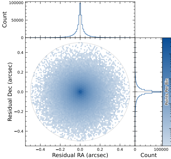
Figure 29. Coordinate residuals for detected synthetic sources in difference images, between recovered and true position of the sources in the ECDFS field. In the top and right panels we include the histogram of these offsets. The circle reflects the matching radius of 0''.5 .
