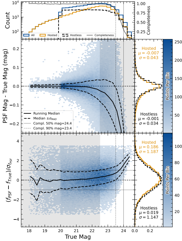
Figure 34. Magnitude residuals and flux pulls for PSF photometry on difference images for ECDFS field in i for detected fake sources. Top panel: Distribution of true magnitudes for injected sources (blue), also splitting into hostless (black dash) and hosted (orange) sources, with detection completeness as a function of true magnitude (gray line). Vertical dashed lines indicate the 90% and 50% completeness limits. Center left panel: 2D hexbin plot of PSF magnitude residuals (measured minus true) versus true magnitude for detected sources, with running median (solid black) and \sigma_{MAD} (dashed black) overlaid. Center right panel: Marginalized distributions of PSF magnitude residuals for hostless (blue) and hosted (orange) sources with true magnitude m_i < 22.5 , annotated with robust mean and standard deviation. Bottom left panel: 2D hexbin plot of PSF flux pulls versus true magnitude for detected sources, with running median (solid black) and \sigma_{MAD} (dashed black) overlaid. Bottom right panel: Marginalized distributions of PSF flux pulls for hostless (blue) and hosted (orange) sources with true magnitude m_i < 22.5 , annotated with robust mean and standard deviation.
