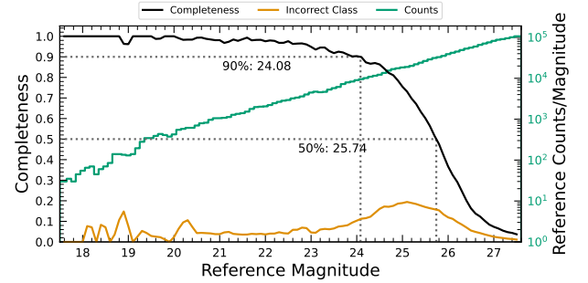
Figure 25. Completeness and incorrect classification fraction as a function of i -band CModel magnitude for DC2-based injected objects into a portion of the ECDFS field. The "Incorrect Class" line shows the proportion of objects that are matched but classified incorrectly by their reference-band extendedness, i.e. stars with extendedness of 1 or galaxies with extendedness of 0 in the reference band.
