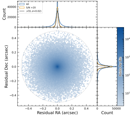
Figure 33. Coordinate residuals for detected synthetic sources in difference images, between recovered and true position of the sources in the ECDIFS field. In the top and right panels we include the distribution of these offsets, for all sources as well as for sources with S/N > 20 . These high S/N sources show gaussian coordinate residual distributions with \sigma = 0''.02 (black solid lines). The circle reflects the matching radius of 0''.5 .
