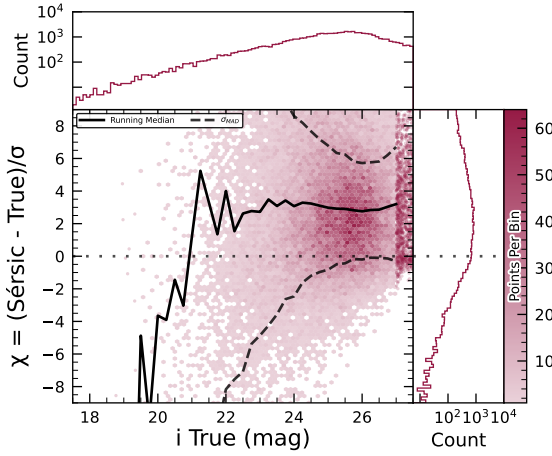
(a) i -band magnitude uncertainty-scaled residuals for Sérsic model measurements of injected galaxies.
