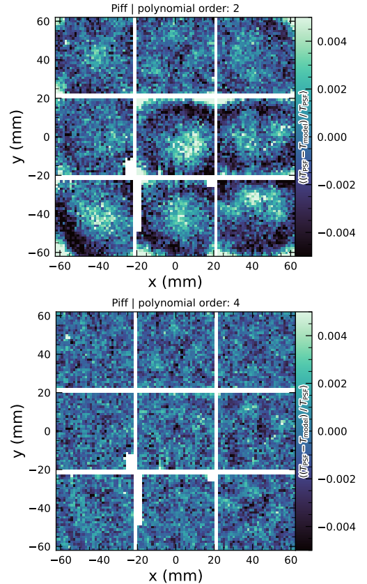
Figure 14. Average across all visits of \delta T/T for Piff O2 and Piff O4 modeling on LSSTComCam. Averages are computed using a 120 \times 120 binning.
