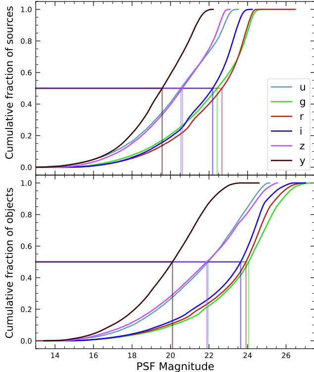
Figure 9. Normalized cumulative histograms of the PSF magnitudes of all > 5\sigma -detected sources (top panel) and objects (bottom panel) contained in the Source and Object catalogs, respectively, separated according to band (see legend). The vertical lines indicate the 50th percentile for each band.
