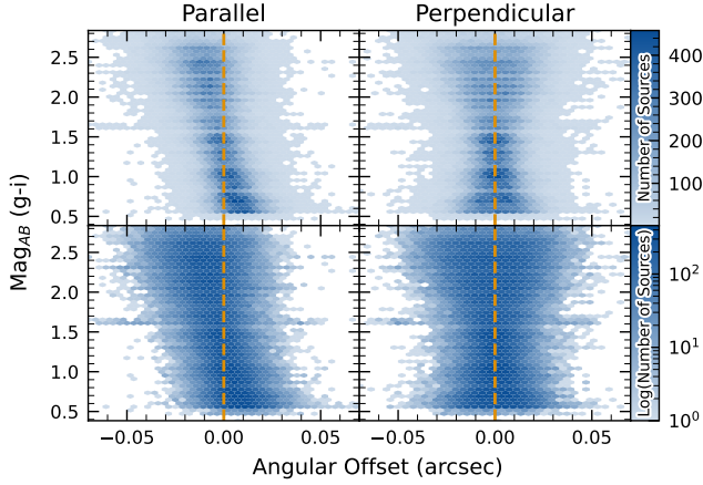
Figure 26. Visualization of Differential Chromatic Refraction (DCR) observed in the LSSTComCam commissioning campaign. The g - i color is computed for every source in the reference catalog (§3.3.3) that is matched to a direct source in the science image, and the binned density for the full survey is plotted against the angular offset between the reference and detected positions. The angular offset is projected along coordinates parallel and perpendicular to the parallactic angle of the observation, and shows a characteristic correlation along the parallel axis with no correlation along the perpendicular axis. The orange vertical dashed line indicates the expected g - i magnitude distribution at zero angular offset.
