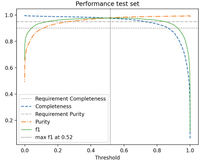
Figure 36. The purity and completeness of the reliability score is shown as a function of reliability threshold based on the testing data. A vertical line marks the threshold where the highest F1-score is obtained. The F1 score is the harmonic mean of completeness and purity. See §4.6.1 for details on the model and model training.
