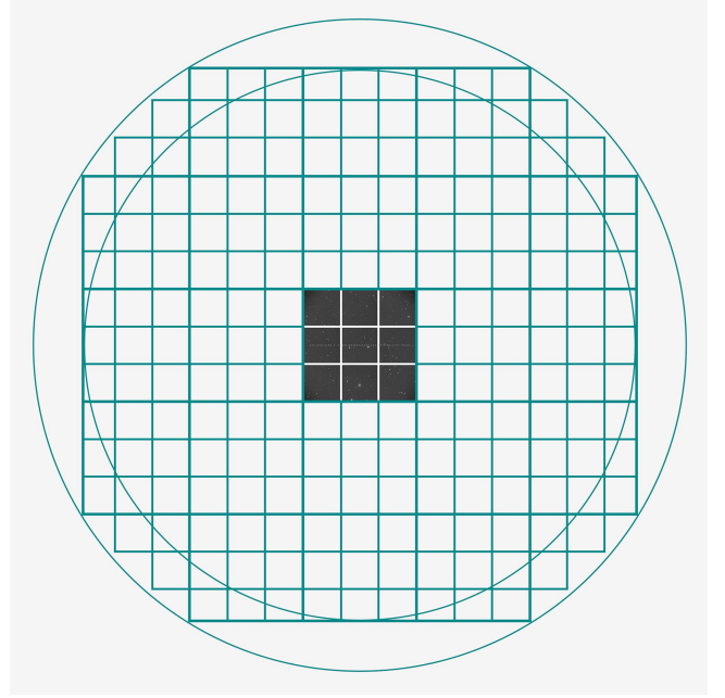
Figure 1. LSSTComCam focal plane layout illustrating the placement of its nine sensors, shown in gray, which form a raft. The view is looking down from above the focal plane through the LSSTComCam lenses. LSSTComCam is Raft 22 (R22). We also indicate the location of the LSSTCam sensors (open squares) to highlight the field-of-view of LSSTComCam in relation to that of LSSTCam .
