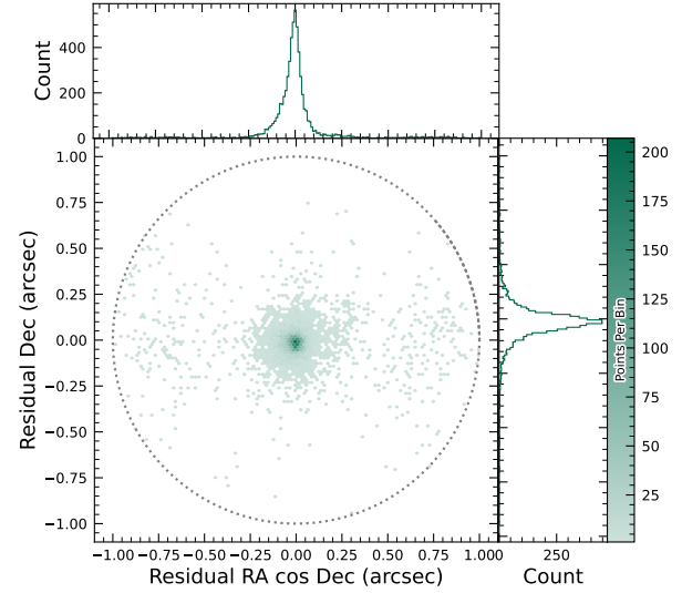
Figure 31. Astrometric residuals between expected and observed positions of SSOs in DP1 . The median residuals are 0''.001 and -0''.016 in R.A./Dec direction, with the standard deviations of 0''.19 and 0''.10 , respectively. No detectable detectable systematic offset from zero indicates there are no major errors in either timing or astrometry delivered by the Rubin system. The wider scatter in the RA-direction is due to objects whose measured orbital elements are less well constrained, translating to larger along-track positional errors in the predicted positions.
