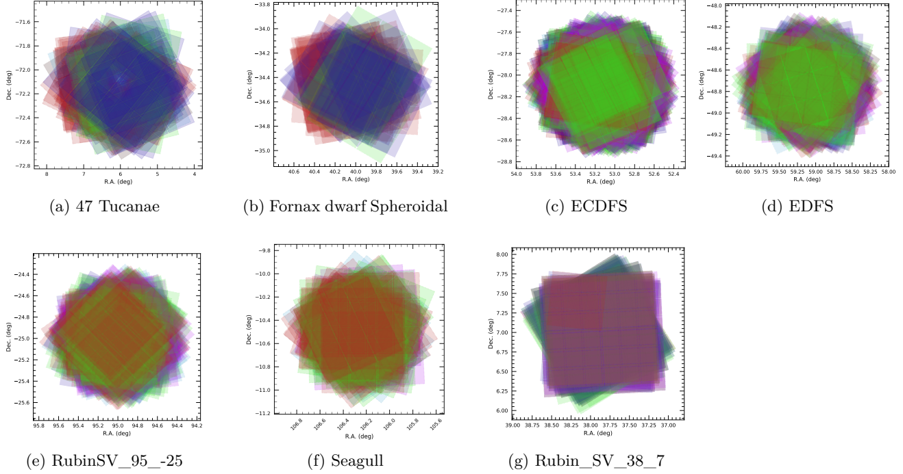
Figure 6. Sky coverage for seven DP1 fields.
