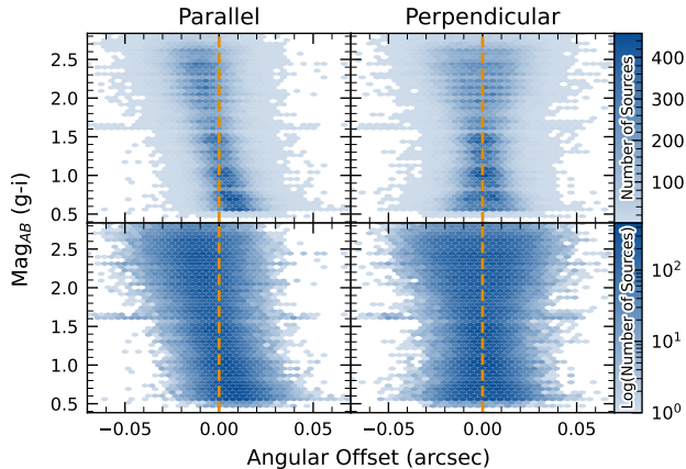
Figure 27. Visualization of Differential Chromatic Refraction (DCR) observed in the LSSTComCam commissioning campaign. The g - i color is computed for every source in the reference catalog that is matched to a direct source in the science image, and the binned density for the full survey is plotted against the angular offset between the reference and detected positions. The angular offset is projected along coordinates parallel and perpendicular to the parallactic angle of the observation, and shows a characteristic correlation along the parallel axis with no correlation along the perpendicular axis. The orange vertical dashed line indicates the expected g - i magnitude distribution at zero angular offset, while the green ‘x’ marks the average g - i magnitude of the plotted sources.
