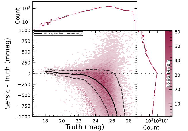
Figure 25. Magnitude residuals for matched injected galaxies with the CModel and Sersic algorithms.
