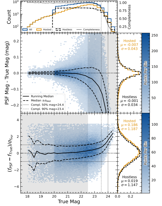
Figure 34. Magnitude residuals and flux pulls for i -band PSF photometry on difference images for ECDFS field in i for detected injected sources. Top panel: Distribution of true magnitudes for injected sources (blue), and split into hostless (black dash) and hosted (orange) sources, with detection completeness as a function of true magnitude (gray line). Vertical dashed lines indicate the 90% and 50% completeness magnitude limits. Center left panel: 2D hexbin plot of PSF magnitude residuals (measured minus true) versus true magnitude for detected sources, with running median (solid black) and \sigma_{MAD} (dashed black) overlaid. Center right panel: Marginalized distributions of PSF magnitude residuals for hostless (blue) and hosted (orange) sources with true magnitude m_i < 22.5 , annotated with robust mean and standard deviation. Bottom left panel: 2D hexbin plot of PSF flux pulls versus true magnitude for detected sources, with running median (solid black) and \sigma_{MAD} (dashed black) overlaid. Bottom right panel: Marginalized distributions of PSF flux pulls for hostless (blue) and hosted (orange) sources with true magnitude m_i < 22.5 , annotated with robust mean and standard deviation.
