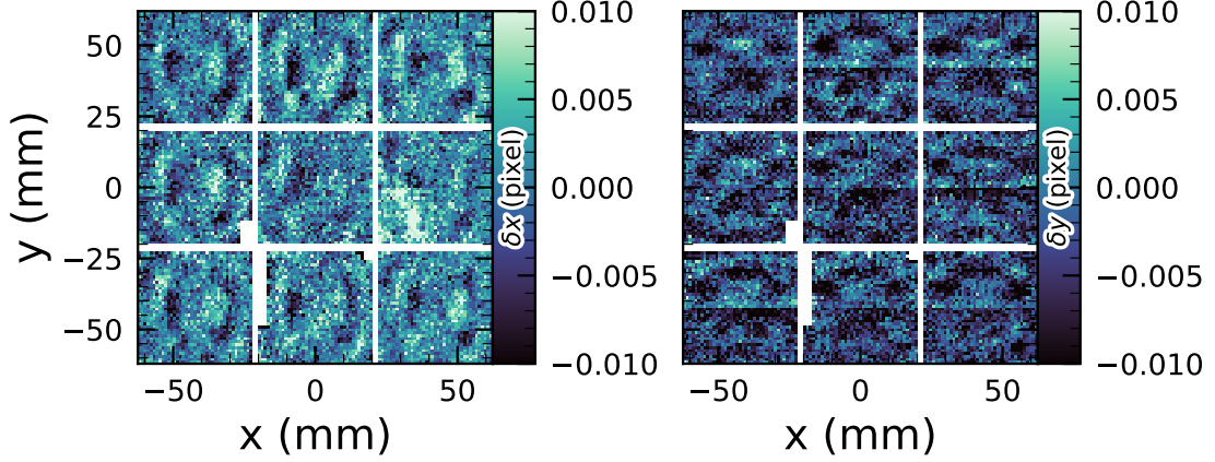
Figure 22. Median astrometric residuals as a function of focal plane position, shown in the left panel for the x direction and in the right panel for the y direction, for all nine LSSTComCam CCDs independently. The range of the color scale is \pm 0.01 pixels, corresponding to 2 mas, showing that the effect is small.
