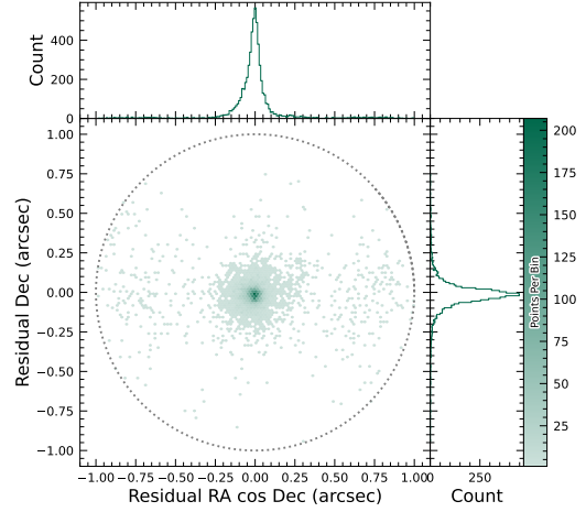
Figure 35. Astrometric residuals between expected and observed positions of Solar System Objects in DP1. The median residuals are 0''.001 and -0''.016 in R.A./Dec direction, with standard deviations of 0''.19 and 0''.10 , respectively. No detectable systematic offset from zero indicates there are no major errors in either timing or astrometry delivered by the Rubin system. The wider scatter in the RA direction is due to objects whose measured orbital elements are less well constrained, translating to larger along-track positional errors in the predicted positions.
