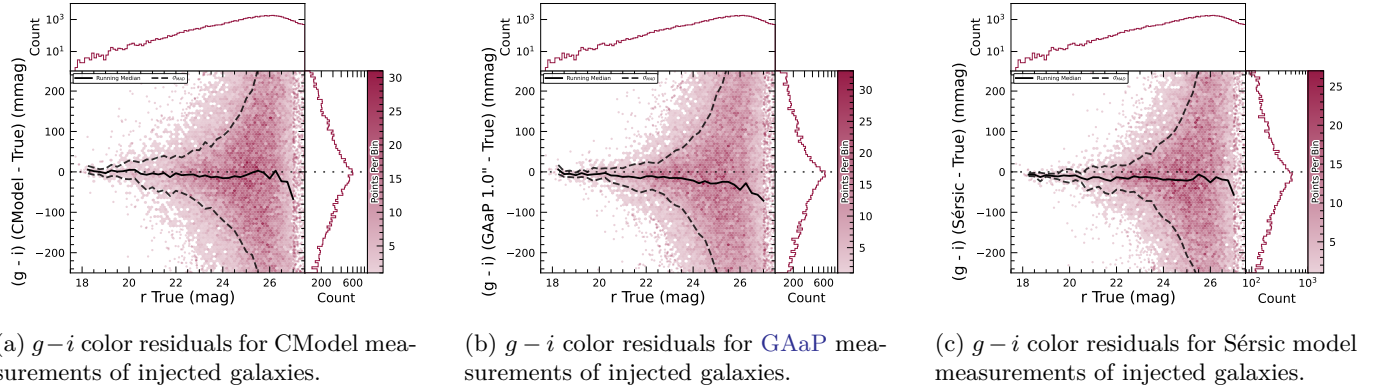
Figure 28. g-i color residuals versus true r -band magnitude for matched injected DC2 galaxies with the CModel, GAAP and Sérsic algorithms in a portion of the ECDFS region.
