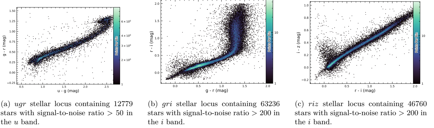
Figure 25. Examples of stellar loci from the full DP1 data set.
