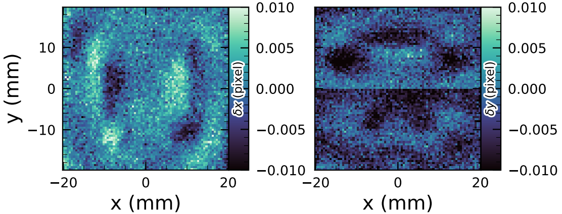
Figure 23. Median residuals as a function of pixel position, shown in the left panel for the x direction and in the right panel for the y direction. These residuals are aggregated across all nine CCDs that comprise the central LSSTComCam raft. The range of the color scale is \pm 0.01 pixels, corresponding to 2 mas, showing that the effect is small.
