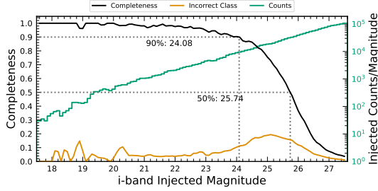
Figure 26. Completeness and incorrect classification fraction as a function of i -band CModel magnitude (Reference Magnitude) for DC2-based injected objects into a portion of the ECDFS field. The “Incorrect Class” line shows the proportion of objects that are matched but classified incorrectly by their reference-band extendedness, i.e. stars with extendedness of 1 or galaxies with extendedness of 0 in the reference band.
