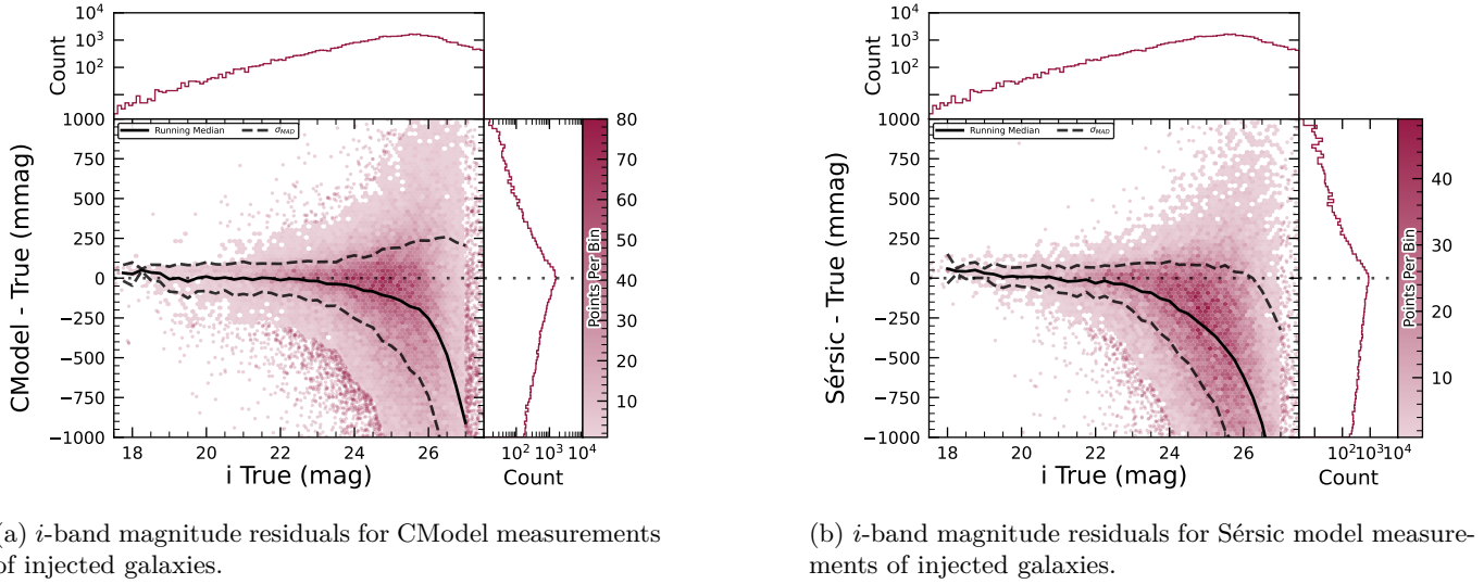
Figure 27. i -band magnitude residuals for matched injected DC2 galaxies with the CModel and Sérsic algorithms in a portion of the ECDFS region, including the median and scatter thereof. The black line is the median.
