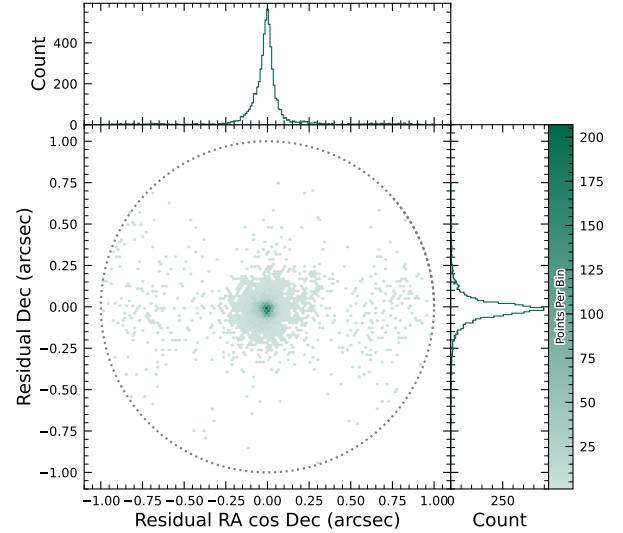
Figure 34. Astrometric residuals between expected and observed positions of SSOs in DP1 . The median residuals are 0.''001 and -0.''016 in R.A./Dec direction, with the standard deviations of 0.''19 and 0.''10 , respectively. No detectable systematic offset from zero indicates there are no major errors in either timing or astrometry delivered by the Rubin system. The wider scatter in the RA-direction is due to objects whose measured orbital elements are less well constrained, translating to larger along-track positional errors in the predicted positions.
