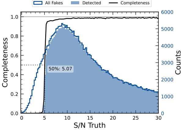
Figure 31. The difference image detection completeness for injected sources in the ECDFS field, for filters griz , as function of the estimated signal to noise ratio S/N. This completeness is the ratio between the found fake sources (shaded histogram) and all the sources (solid line). The horizontal dashed line represents where the 50% completeness level is reached, at approximately S/N \simeq 5.07 .
