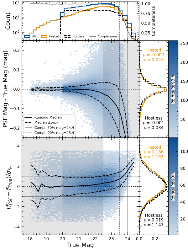
Figure 33. Magnitude residuals and flux pulls for PSF photometry on difference images for ECDFS field in i for detected fake sources. Top panel: Distribution of true magnitudes for injected sources (blue), also splitting into hostless (black dash) and hosted (orange) sources, with detection completeness as a function of true magnitude (gray line). Vertical dashed lines indicate the 90% and 50% completeness magnitude limits. Center left panel: 2D hexbin plot of PSF magnitude residuals (measured minus true) versus true magnitude for detected sources, with running median (solid black) and \sigma_{MAD} (dashed black) overlaid. Center right panel: Marginalized distributions of PSF magnitude residuals for hostless (blue) and hosted (orange) sources with true magnitude m_i < 22.5 , annotated with robust mean and standard deviation. Bottom left panel: 2D hexbin plot of PSF flux pulls versus true magnitude for detected sources, with running median (solid black) and \sigma_{MAD} (dashed black) overlaid. Bottom right panel: Marginalized distributions of PSF flux pulls for hostless (blue) and hosted (orange) sources with true magnitude m_i < 22.5 , annotated with robust mean and standard deviation.
