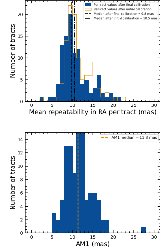
Figure 17. (a) Mean per-tract astrometric repeatability of measurements of isolated point sources in Rapid Analysis (RA) (b) Median per-tract repeatability in separations between isolated point sources 5 arcmin apart.
