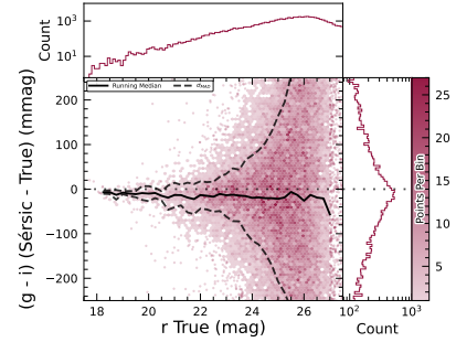
(c) g-i color residuals for Sérsic model measurements of injected galaxies.
