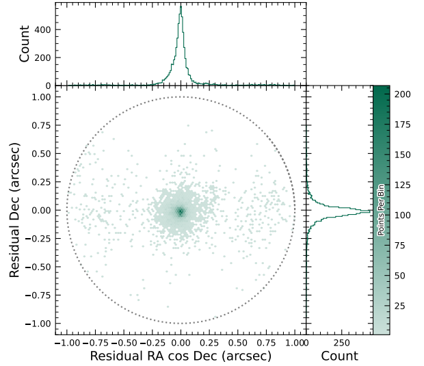
Figure 34. Astrometric residuals between expected and observed positions of SSOs in DP1. The median residuals are 0.''001 and -0.''016 in R.A./Dec direction, with the standard deviations of 0.''19 and 0.''10 , respectively. No detectable systematic offset from zero indicates there are no major errors in either timing or astrometry delivered by the Rubin system. The wider scatter in the RA-direction is due to objects whose measured orbital elements are less well constrained, translating to larger along-track positional errors in the predicted positions.
