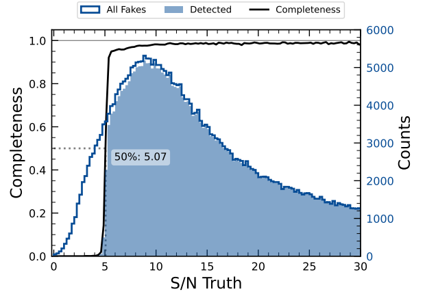
Figure 31. The difference image detection completeness for injected sources in the ECDFS field, for filters griz , as function of the estimated signal to noise ratio S/N. This completeness is the ratio between the found fake sources (shaded histogram) and all the sources (solid line). The horizontal dashed line represents where the 50% completeness level is reached, at approximately S/N \simeq 5.07 .
