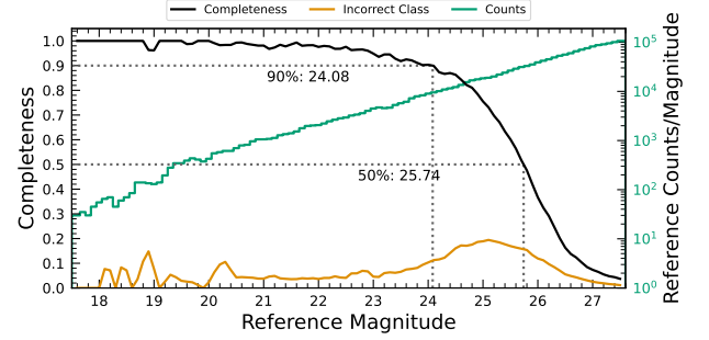
Figure 24. Completeness as a function of i -band CModel magnitude for DC2 -based injected objects into a portion of the ECDFS field. The “Incorrect Class” line shows the proportion of objects that are matched but classified incorrectly by their reference-band extendedness, i.e. stars with extendedness of 1 or galaxies with extendedness of 0 in the reference band.
