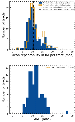
Figure 17. (a) Mean per-tract astrometric repeatability of measurements of isolated point sources in Right Ascension (RA) (b) Median per-tract repeatability in separations between isolated point sources 5 arcmin apart.
