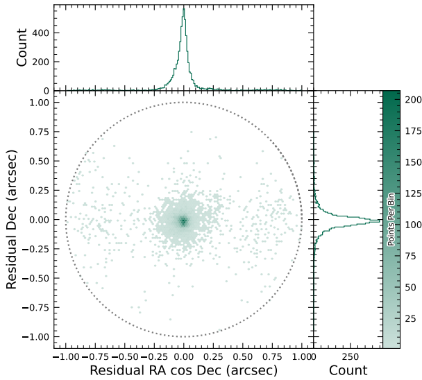
Figure 39. Astrometric residuals between expected and observed positions of Solar System Objects in DP1. The median residuals are 0''.001 and -0''.016 in R.A./Dec direction, with standard deviations of 0''.19 and 0''.10 , respectively. No detectable systematic offset from zero indicates there are no major errors in either timing or astrometry delivered by the Rubin system. The wider scatter in the RA direction is due to objects whose measured orbital elements are less well constrained, translating to larger along-track positional errors in the predicted positions.
