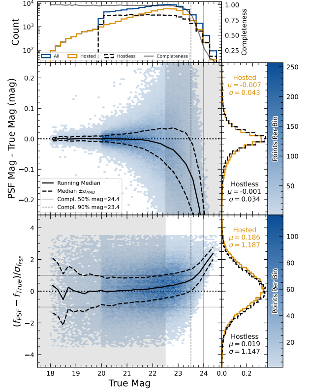
Figure 38. Magnitude residuals and flux pulls for i -band PSF photometry on difference images for ECDFS field in i for detected injected sources. Top panel: Distribution of true magnitudes for injected sources (blue), and split into hostless (black dash) and hosted (orange) sources, with detection completeness as a function of true magnitude (gray line). Vertical dashed lines indicate the 90% and 50% completeness magnitude limits. Center left panel: 2D hexbin plot of PSF magnitude residuals (measured minus true) versus true magnitude for detected sources, with running median (solid black) and \sigma_{MAD} (dashed black) overlaid. Center right panel: Marginalized distributions of PSF magnitude residuals for hostless (blue) and hosted (orange) sources with true magnitude m_i < 22.5 , annotated with robust mean and standard deviation. Bottom left panel: 2D hexbin plot of PSF flux pulls versus true magnitude for detected sources, with running median (solid black) and \sigma_{MAD} (dashed black) overlaid. Bottom right panel: Marginalized distributions of PSF flux pulls for hostless (blue) and hosted (orange) sources with true magnitude m_i < 22.5 , annotated with robust mean and standard deviation.
