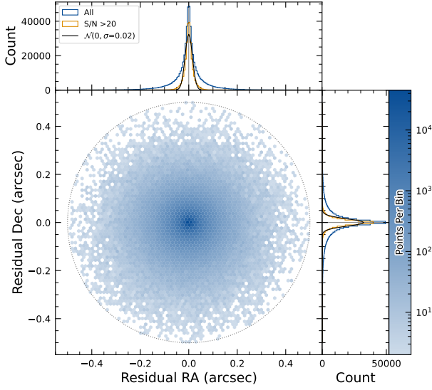
Figure 37. Coordinate residuals for detected synthetic sources in difference images, between recovered and true position of the sources in the ECDFS field. In the top and right panels we include the distribution of these offsets, for all sources as well as for sources with \text{SNR} > 20 . These high SNR sources show gaussian coordinate residual distributions with \sigma = 0''.02 (black solid lines). The circle reflects the matching radius of 0''.5 .
