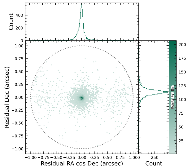
Figure 28. Astrometric residuals between expected and observed positions of SSOs in DP1. The median residuals are 0."001 and −0."016 in R.A./Dec direction, with the standard deviations of 0."19 and 0."10, respectively. No detectable detectable systematic offset from zero indicates there are no major errors in either timing or astrometry delivered by the Rubin system. The wider scatter in the RA-direction is due to objects whose measured orbital elements are less well constrained, translating to larger along-track positional errors in the predicted positions.
