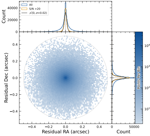
Figure 32. Coordinate residuals for detected synthetic sources in difference images, between recovered and true position of the sources in the ECDFS field. In the top and right panels we include the distribution of these offsets, for all sources as well as for sources with S/N > 20 . These high S/N sources show gaussian coordinate residual distributions with \sigma = 0''.02 (black solid lines). The circle reflects the matching radius of 0''.5 .
