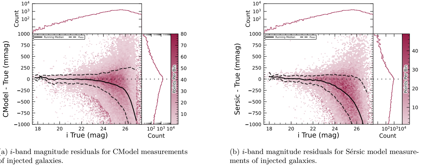
Figure 25. i -band magnitude residuals for matched injected DC2 galaxies with the CModel and Sérsic algorithms in a portion of the ECDFS region.
