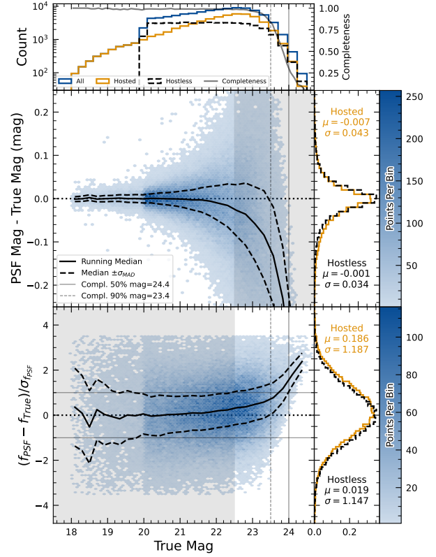
Figure 33. Magnitude residuals and flux pulls for PSF photometry on difference images for ECDFS field in i for detected fake sources. Top panel: Distribution of true magnitudes for injected sources (blue), also splitting into hostless (black dash) and hosted (orange) sources, with detection completeness as a function of true magnitude (gray line). Vertical dashed lines indicate the 90% and 50% completeness magnitude limits. Center left panel: 2D hexbin plot of PSF magnitude residuals (measured minus true) versus true magnitude for detected sources, with running median (solid black) and \sigma_{MAD} (dashed black) overlaid. Center right panel: Marginalized distributions of PSF magnitude residuals for hostless (blue) and hosted (orange) sources with true magnitude m_i < 22.5 , annotated with robust mean and standard deviation. Bottom left panel: 2D hexbin plot of PSF flux pulls versus true magnitude for detected sources, with running median (solid black) and \sigma_{MAD} (dashed black) overlaid. Bottom right panel: Marginalized distributions of PSF flux pulls for hostless (blue) and hosted (orange) sources with true magnitude m_i < 22.5 , annotated with robust mean and standard deviation.
