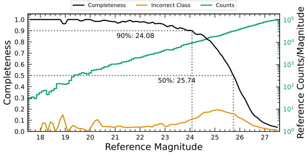
Figure 24. Completeness as a function of i -band CModel magnitude for DC2-based injected objects into a portion of the ECDfS field. The "Incorrect Class" line shows the proportion of objects that are matched but classified incorrectly by their reference-band extendedness, i.e. stars with extendedness of 1 or galaxies with extendedness of 0 in the reference band.
