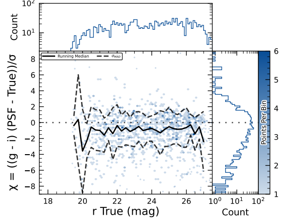
(b) g - i color uncertainty-scaled residuals for PSF model measurements of injected stars.
