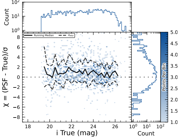
(a) i -band magnitude uncertainty-scaled residuals for PSF model measurements of injected stars.
