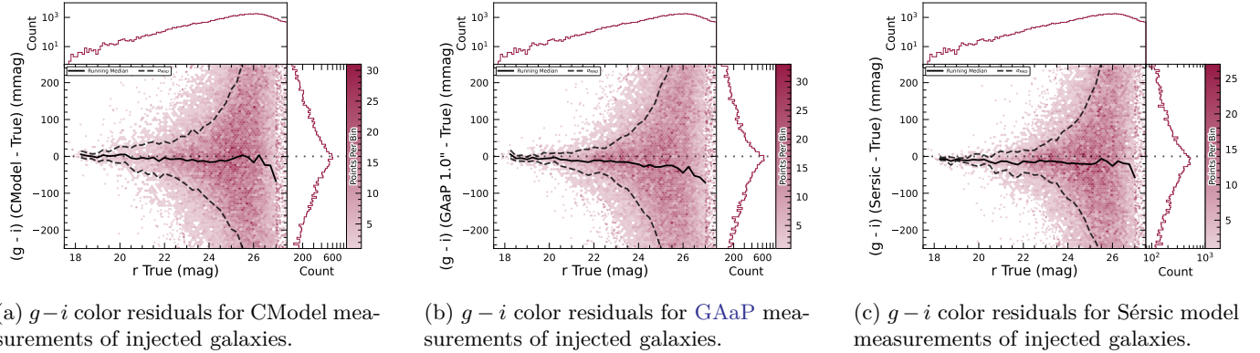
Figure 26. g-i color residuals versus r -band magnitude for matched injected DC2 galaxies with the CModel, GAAP and Sérsic algorithms in a portion of the ECDFS region.
