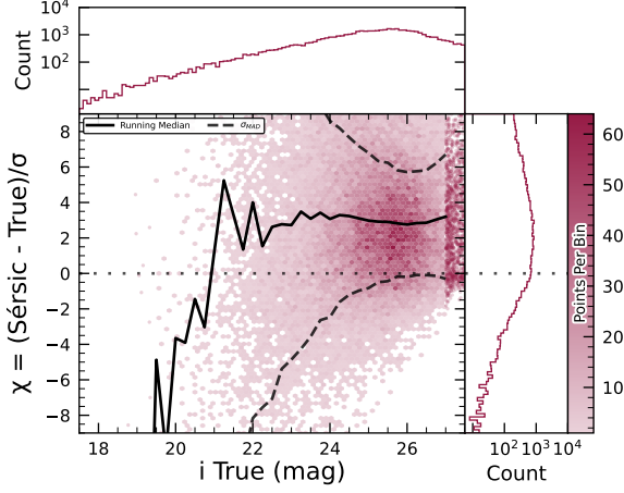
(a) i -band magnitude uncertainty-scaled residuals for Sérsic model measurements of injected galaxies.
