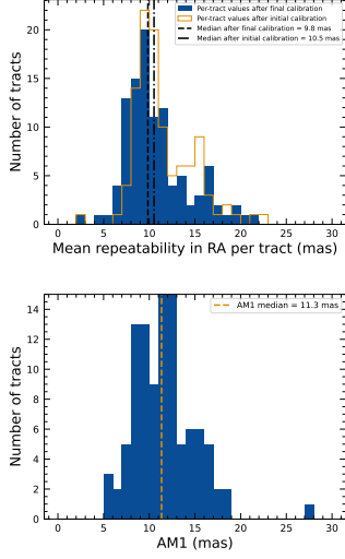
Figure 17. (a) Mean per-tract astrometric repeatability of measurements of isolated point sources in Rapid Analysis (RA) (b) Median per-tract repeatability in separations between isolated point sources 5 arcmin apart.
