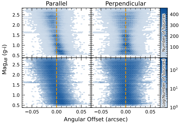
Figure 30. Visualization of Differential Chromatic Refraction (DCR) observed in the LSSTComCam commissioning campaign. The g-i color is computed for every source in the reference catalog that is matched to a direct source in the science image, and the binned density for the full survey is plotted against the angular offset between the reference and detected positions. The angular offset is projected along coordinates parallel and perpendicular to the parallactic angle of the observation, and shows a characteristic correlation along the parallel axis with no correlation along the perpendicular axis. The orange vertical dashed line indicates the expected g-i magnitude distribution at zero angular offset.
