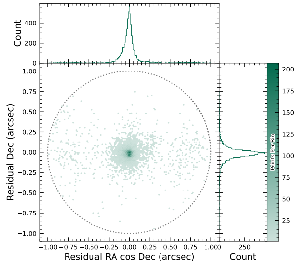
Figure 34. Astrometric residuals between expected and observed positions of SSOs in DP1 . The median residuals are 0.''001 and -0.''016 in RA ./ Dec direction, with the standard deviations of 0.''19 and 0.''10 , respectively. No detectable systematic offset from zero indicates there are no major errors in either timing or astrometry delivered by the Rubin system. The wider scatter in the RA -direction is due to objects whose measured orbital elements are less well constrained, translating to larger along-track positional errors in the predicted positions.
