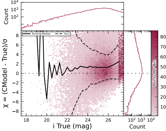
(a) i -band magnitude uncertainty-scaled residuals for CModel measurements of injected galaxies.
