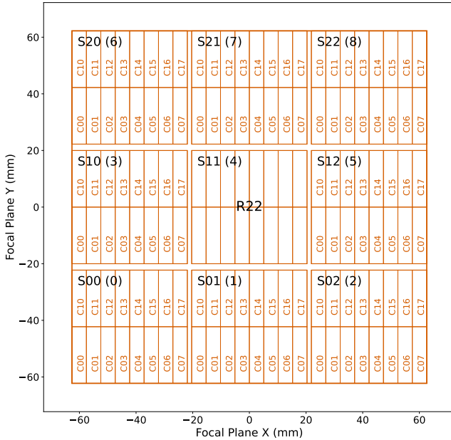
Figure 2. LSSTComCam focal plane layout illustrating the placement and numbering scheme of sensors (S) and amplifiers (C). The view is looking down from above the focal plane through the LSSTComCam lenses. Each sensor contains 16 amplifiers, and a group of nine sensors comprises one raft. LSSTComCam is Raft 22 (R22). The detector number for each sensor is shown in parentheses.
