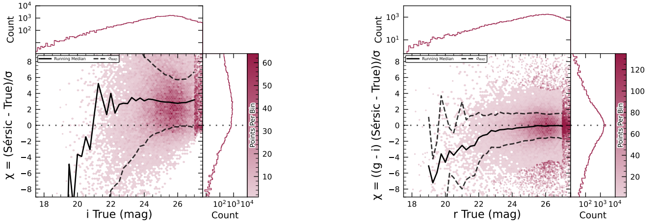
(a) i -band flux uncertainty-scaled residuals for Sérsic model measurements of injected galaxies.
