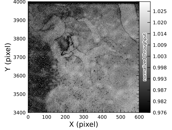
Figure 11. The top left corner of R22_S01 in the g -band flat, showing the many small defect features that are caused by the remnant photoresist wax. A single large defect box masks this region from further analysis to prevent these features from contaminating measurements.
