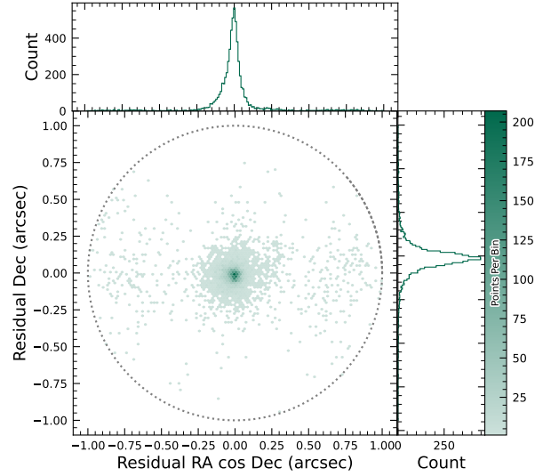
Figure 28. Astrometric residuals between expected and observed positions of SSOs in DP1 . The median residuals are 0''.001 and -0''.016 in RA / Dec direction, with the standard deviations of 0''.19 and 0''.10 , respectively. No detectable detectable systematic offset from zero indicates there are no major errors in either timing or astrometry delivered by the Rubin system. The wider scatter in the RA -direction is due to objects whose measured orbital elements are less well constrained, translating to larger along-track positional errors in the predicted positions.
