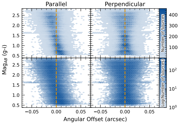
Figure 27. Visualization of Differential Chromatic Refraction (DCR) observed in the LSSTComCam commissioning campaign. The g-i color is computed for every source in the reference catalog that is matched to a direct source in the science image, and the binned density for the full survey is plotted against the angular offset between the reference and detected positions. The angular offset is projected along coordinates parallel and perpendicular to the parallactic angle of the observation, and shows a characteristic correlation along the parallel axis with no correlation along the perpendicular axis. The orange vertical dashed line indicates the expected g-i magnitude distribution at zero angular offset, while the green ‘x’ marks the average g-i magnitude of the plotted sources.
