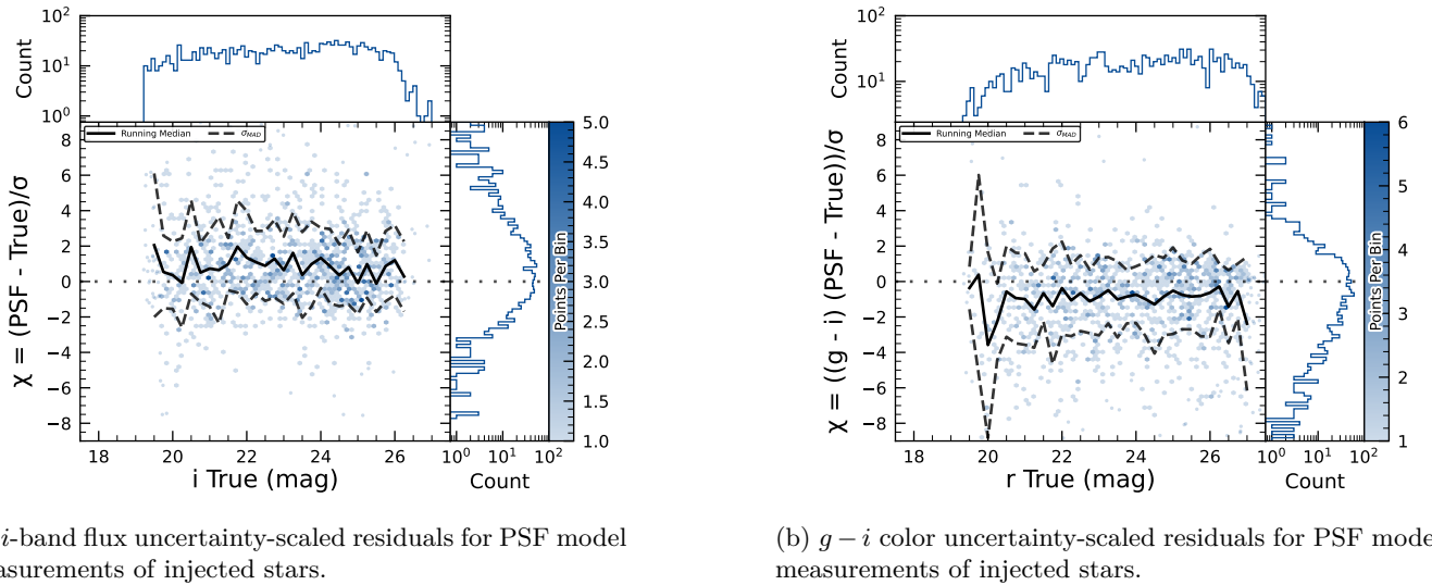
Figure 30. Color and flux uncertainty-scaled residuals for matched injected DC2 stars' PSF model measurements in a portion of the ECDFS region.
