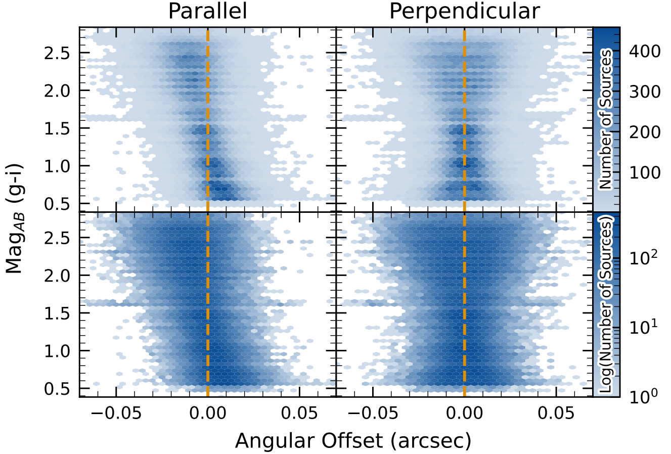
Figure 26. Visualization of Differential Chromatic Refraction (DCR) observed in the LSSTComCam commissioning campaign. The g - i color is computed for every source in the reference catalog that is matched to a direct source in the science image, and the binned density for the full survey is plotted against the angular offset between the reference and detected positions. The angular offset is projected along coordinates parallel and perpendicular to the parallactic angle of the observation, and shows a characteristic correlation along the parallel axis with no correlation along the perpendicular axis. The orange vertical dashed line indicates the expected g - i magnitude distribution at zero angular offset, while the green ‘x’ marks the average g - i magnitude of the plotted sources.
