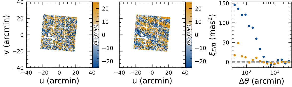
Figure 19. Residuals in du (left panel) and dv (center panel) directions, with the E and B -modes of the two-point correlation function (right panel). The residuals show a wave-like pattern characteristic of atmospheric turbulence, and there is significant E -mode and negligible B -mode in the correlation function.
