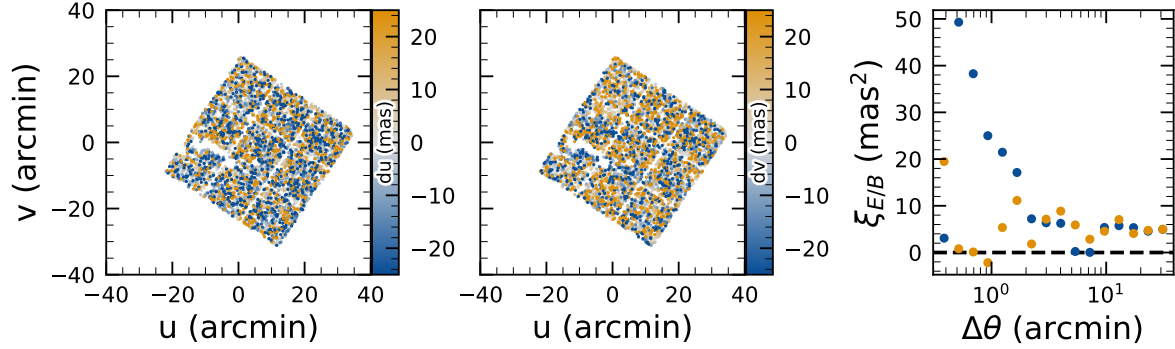
Figure 20. Residuals in du (left panel) and dv (center panel) directions, with the E and B -modes of the two-point correlation function (right panel). There are coherent residuals, but without the wave-like pattern seen in Figure 19, and the correlation function has significant values for both E and B -modes.
