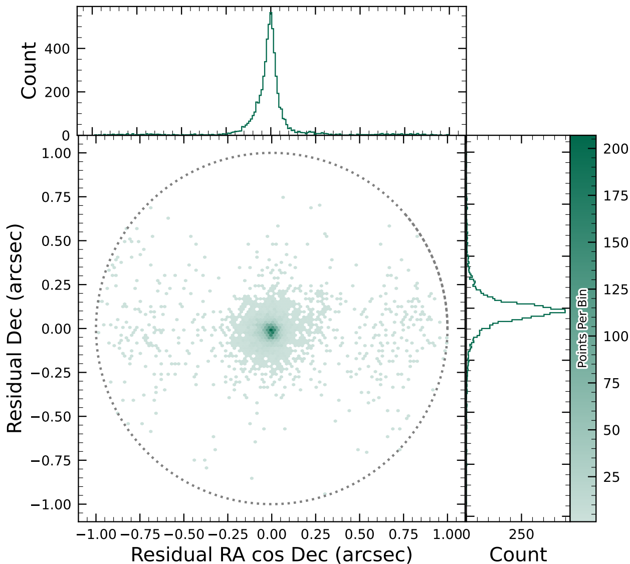
Figure 27. Astrometric residuals between expected and observed positions of SSOs in DP1 . The median residuals are 0.''001 and -0.''016 in R.A./Dec direction, with the standard deviations of 0.''19 and 0.''10 , respectively. No detectable systematic offset from zero indicates there are no major errors in either timing or astrometry delivered by the Rubin system. The wider scatter in the RA-direction is due to objects whose measured orbital elements are less well constrained, translating to larger along-track positional errors in the predicted positions.
