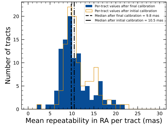
Figure 17. Mean per-tract astrometric repeatability of measurements of isolated point sources in RA in visits across all bands.
