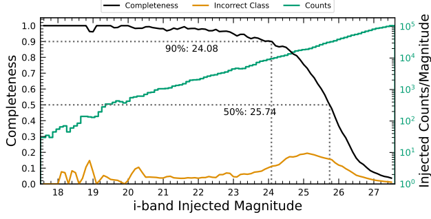
Figure 27. Completeness and incorrect classification fraction as a function of i -band CModel magnitude (Reference Magnitude) for DC2-based injected objects into a portion of the ECDfS field. The “Incorrect Class” line shows the proportion of objects that are matched but classified incorrectly by their reference-band extendedness, i.e. stars with extendedness of 1 or galaxies with extendedness of 0 in the reference band.
