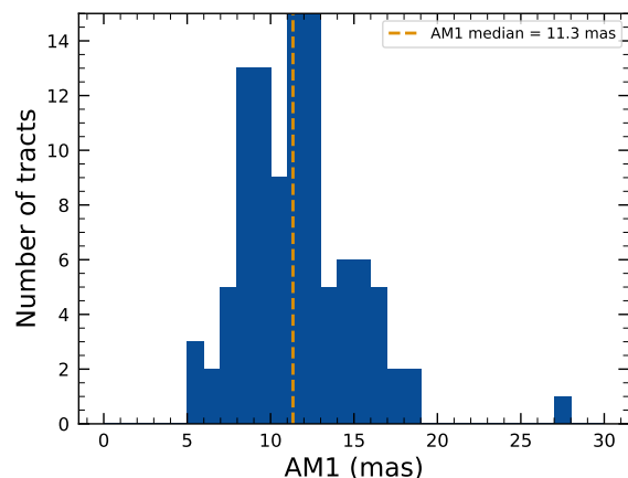
Figure 18. Median per-tract repeatability in separations between isolated point sources 5 arcmin apart in visits across all bands.
