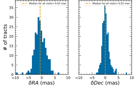
Figure 18. Median absolute offset for all visits in r-band in tract 4849 . The offset is the difference between the position of isolated point sources that were reserved from the astrometric fit and matched objects from the Gaia DR3 catalog.
