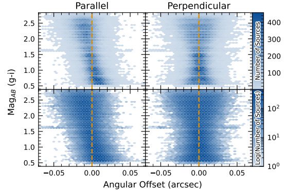
Figure 24. Visualization of Differential Chromatic Refraction (DCR) observed in the LSSTComCam commissioning campaign. The g-i color is computed for every source in the reference catalog that is matched to a direct source in the science image, and the binned density for the full survey is plotted against the angular offset between the reference and detected positions. The angular offset is projected along coordinates parallel and perpendicular to the parallactic angle of the observation, and shows a characteristic correlation along the parallel axis with no correlation along the perpendicular axis. The orange vertical dashed line indicates the expected g-i magnitude distribution at zero angular offset.
